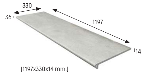
[1197x330x14 mm.]
