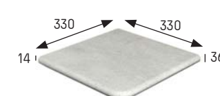
[330x330x14 mm.]
